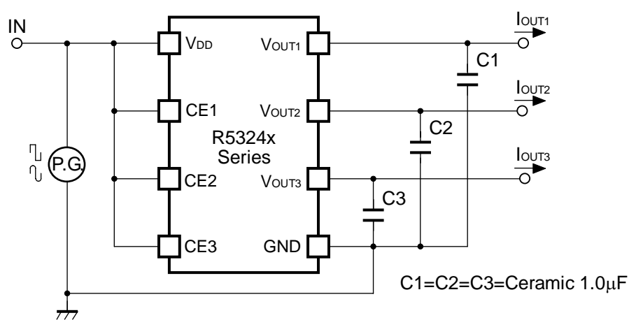
Test Circuit for Ripple Rejection, Input Transient Response
