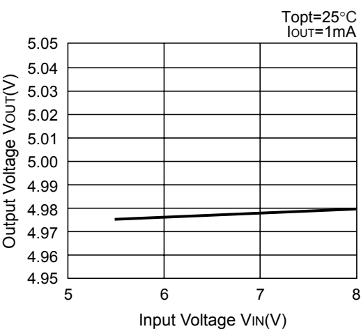
Rx5RW50B
