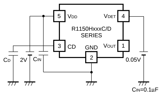
VD Output Current Test Circuit
