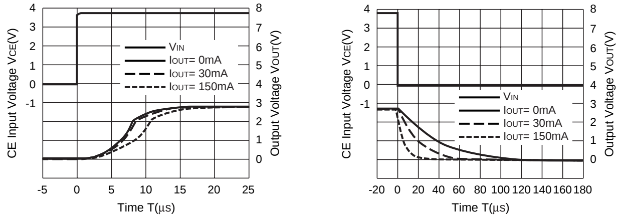
R1114x281D ( V_{IN}=3.8V , C_{IN} =Ceramic 0.47\mu F , C_{OUT} =Ceramic 0.47\mu F )
