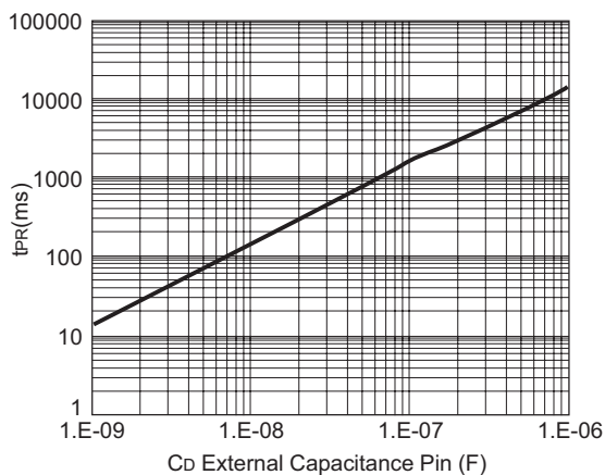
13) tPR vs. External Capacitance of C D Pin
