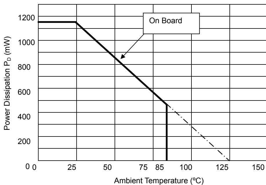
Power Dissipation
