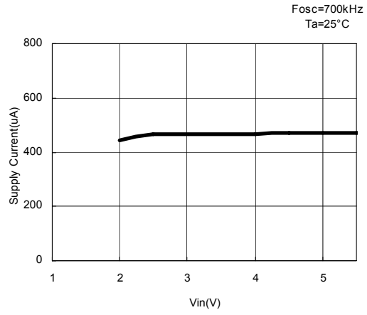
R1290K102A
