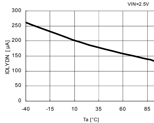
36) DELAY Discharge Current VS. Temperature R1290K102A
