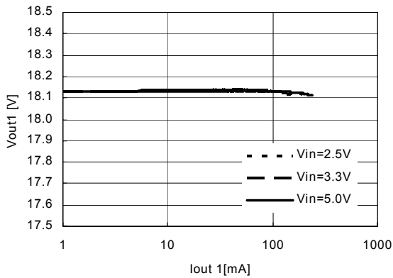
R1290K102A
