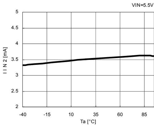
R1290K102A
