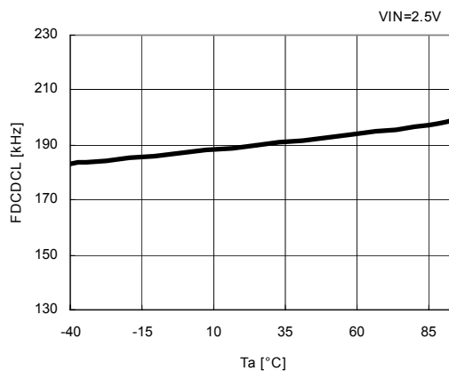
R1290K102A
