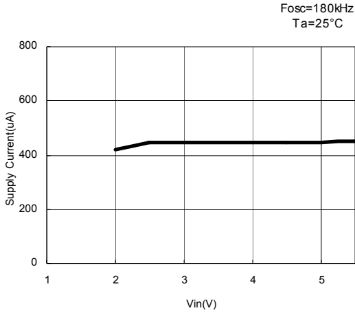
R1290K102A
