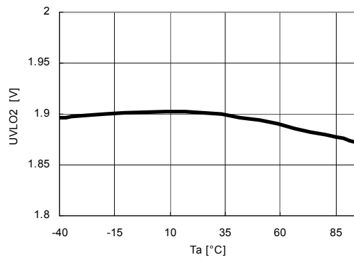
R1290K102A
