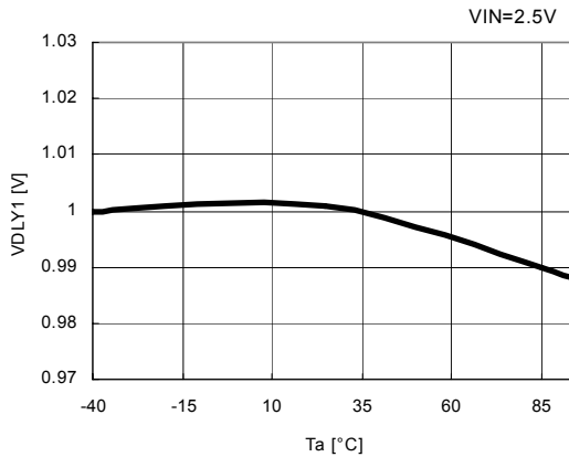
37) DELAY Detector Threshold VS. Temperature R1290K102A
