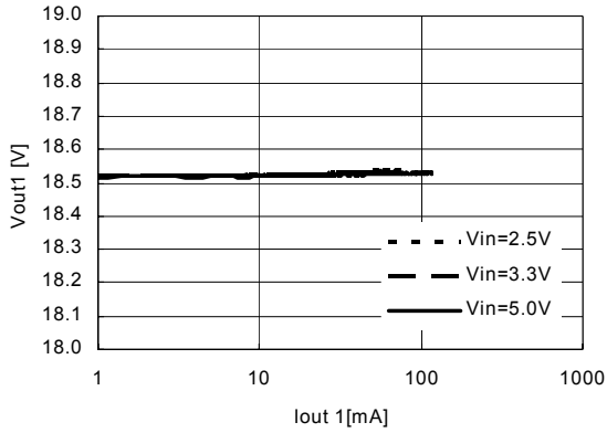
R1290K102A
