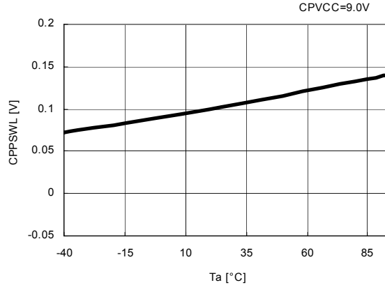
38) CPPSW "L" Output Voltage VS. Temperature R1290K102A
