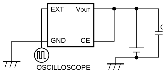
Test Circuit 2
