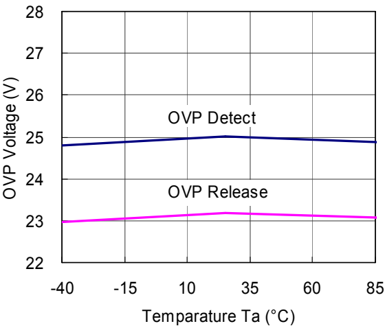
12) OVP Voltage vs. Temperature
