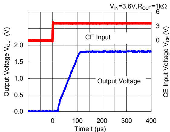
RP502x182B/184B
