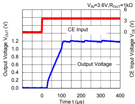
RP502x121B/123B
