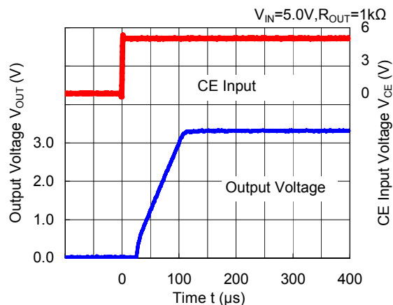
RP502x332B/334B
