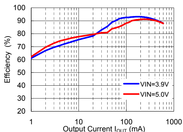
RP502x291B/293B
