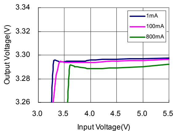
RP501K331x(PWM fixed)
