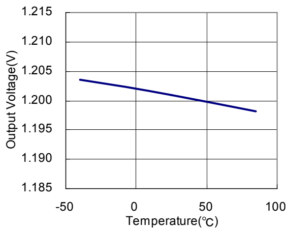
RP501K121x(PWM fixed)
