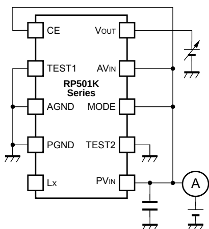
Supply Current 1 / 2
