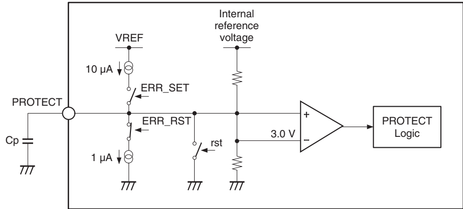
Fig. 14. PROTECT Pin Equivalent Circuit
