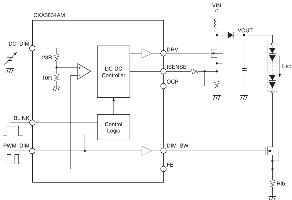
Fig. 3. CXA3834AM Operating Circuit Diagram
