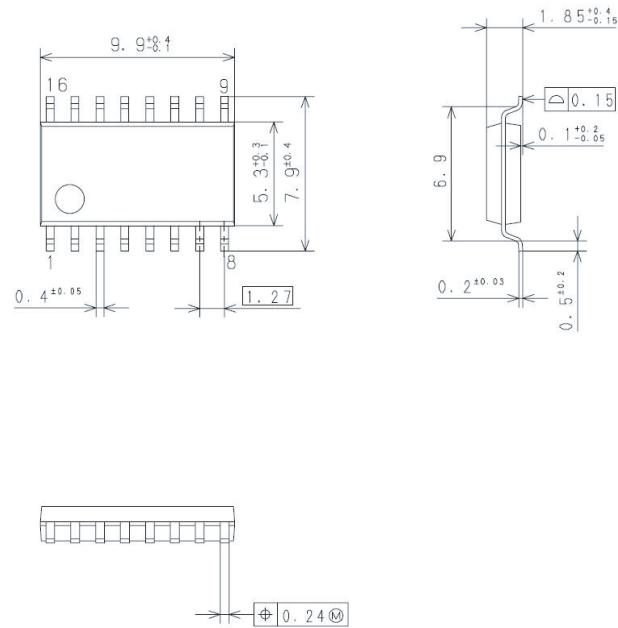
16PIN SOP (PLASSTIC)
