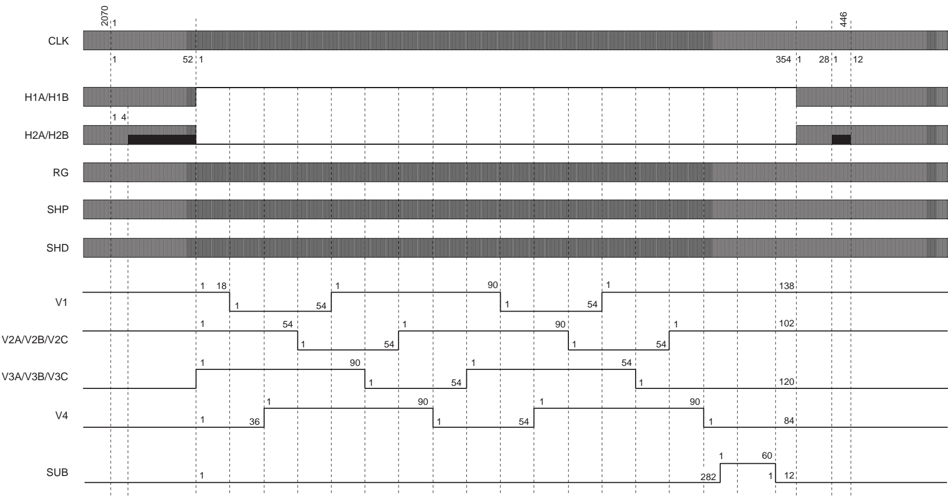
Drive Timing Chart (Horizontal Sync) 2-line Addition Mode
