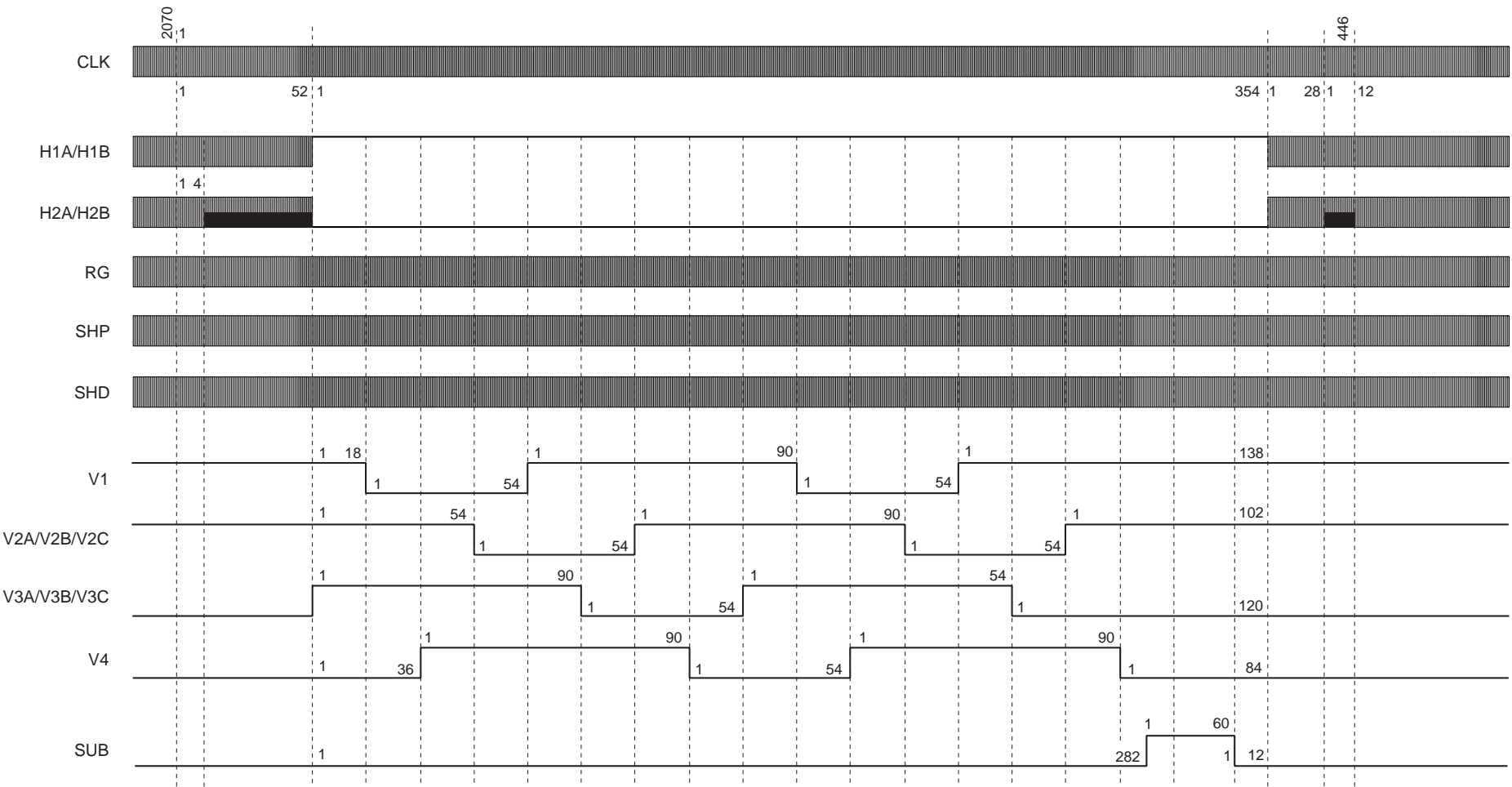
Drive Timing Chart (Horizontal Sync) 2/4-line Readout Mode
