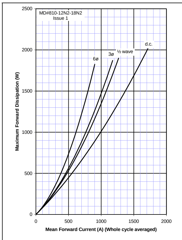
Figure 7 – On-state current vs. Power dissipation
