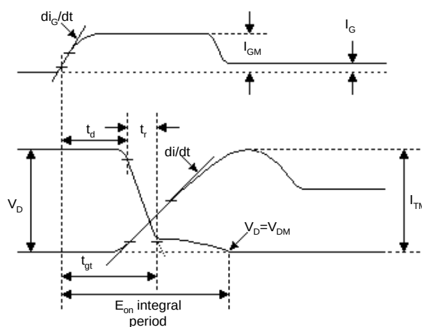
Diagram 9, Turn-on wave-diagrams.
