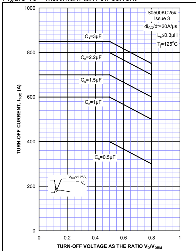
Figure 16 – Maximum turn-off current
