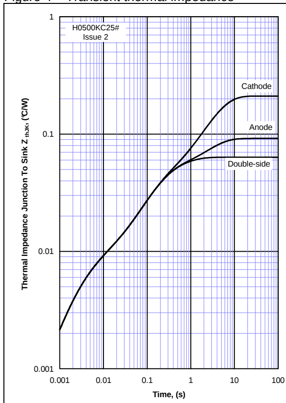
Figure 4 – Transient thermal impedance
