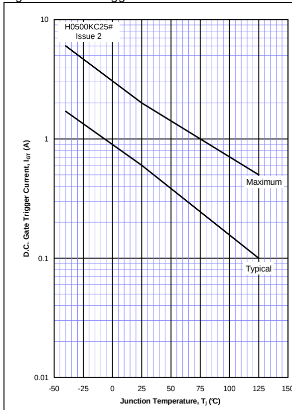
Figure 6 – Gate trigger current
