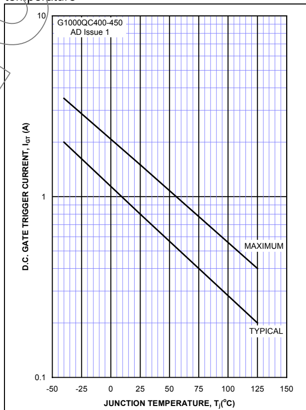
Figure 6 – Gate trigger current Vs junction temperature
