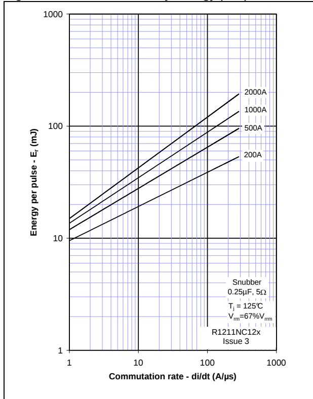
Figure 9 - Reverse recovery energy per pulse
