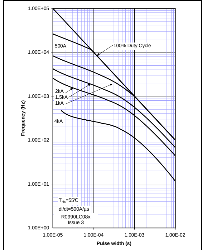
Figure 14 - Square wave frequency ratings
