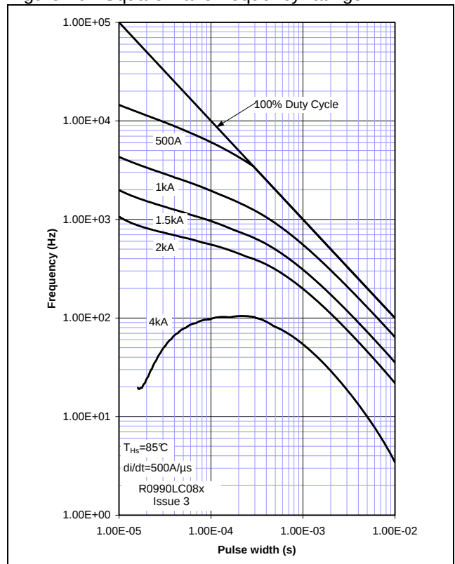
Figure 16 - Square wave frequency ratings
