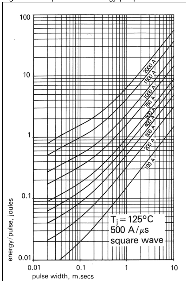
Figure 15 - Maximum reverse recovery energy loss per pulse at T_j = 125^\circ\text{C} and V_{rm} = 536\text{ volts}
