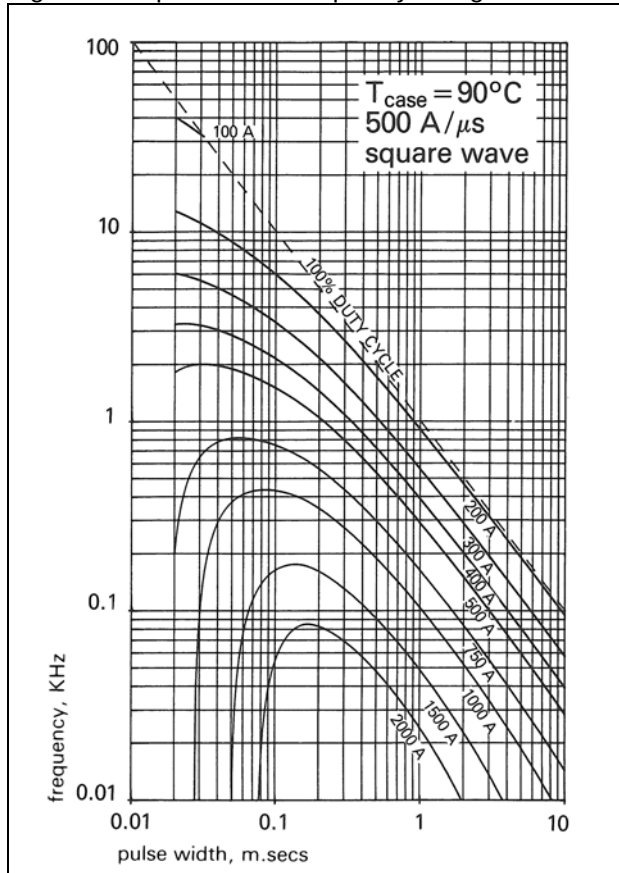
Figure 9 - Square wave frequency ratings
