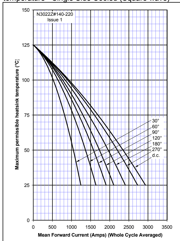
Figure 15 – On-state current vs. Heatsink temperature - Single Side Cooled (Square wave)
