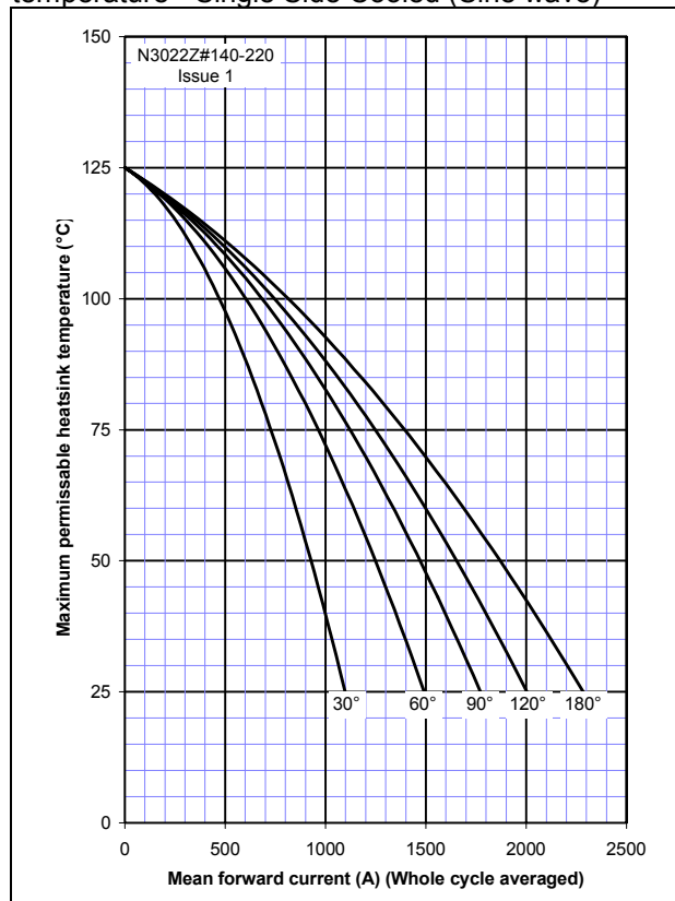
Figure 13 – On-state current vs. Heatsink temperature - Single Side Cooled (Sine wave)
