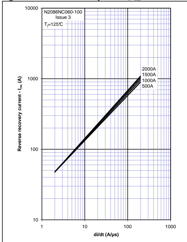
Figure 6 – Reverse recovery current, I_{rm}
