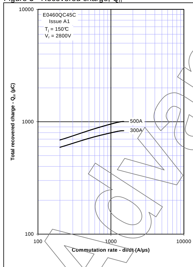
Figure 3 - Recovered charge, Q_{rr}
