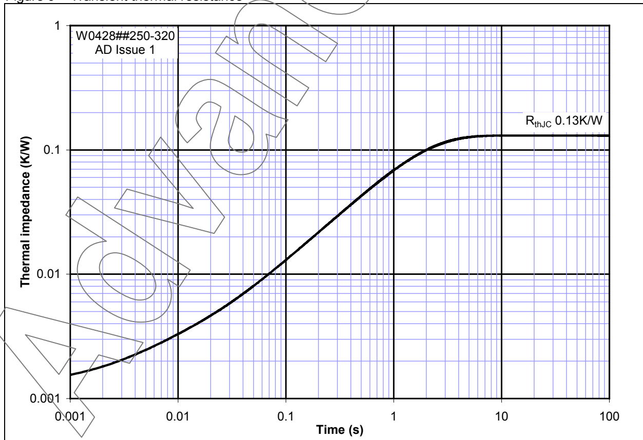
Figure 9 – Transient thermal resistance
