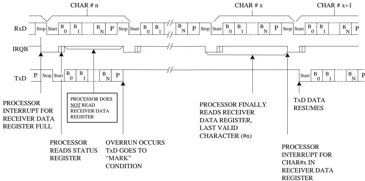
Figure 12 Overrun in Echo Mode
