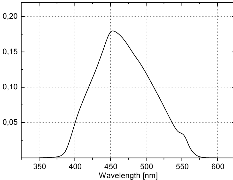
Typical Optical Responsivity (A/W)
