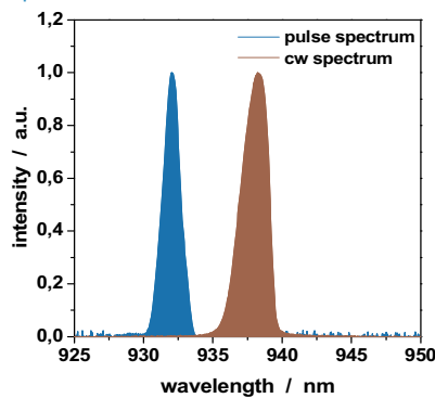
Spectral Characteristic*
