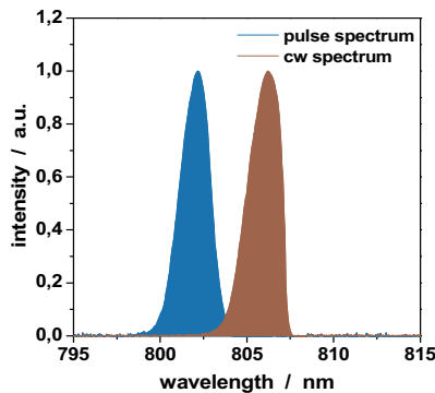
Spectral Characteristic*
