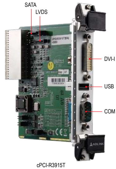
cPCI-R3915T
