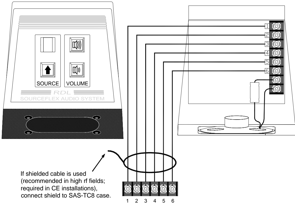
Connection to SourceFlex controller SAS-8C, SAS-8i or SAS-82
