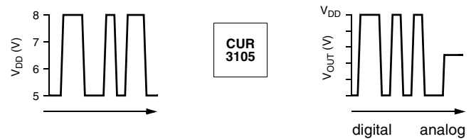
Fig. 2-1: Programming with V_{DD} modulation
