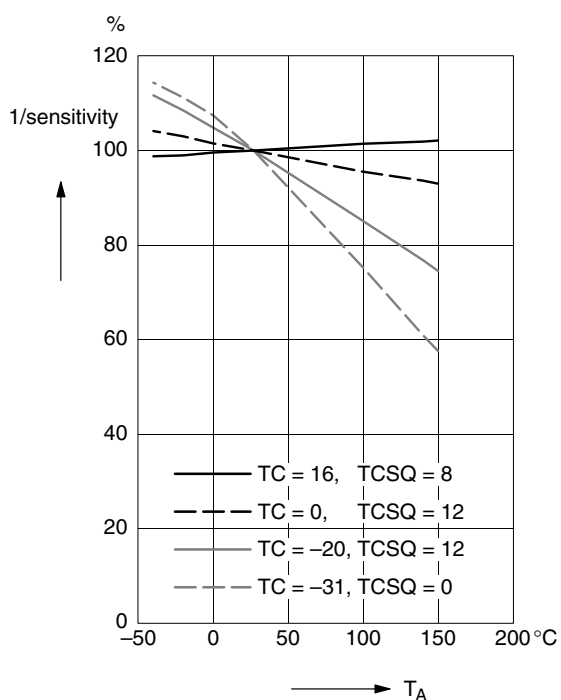
Fig. 3-8: Typical 1/sensitivity versus ambient temperature
