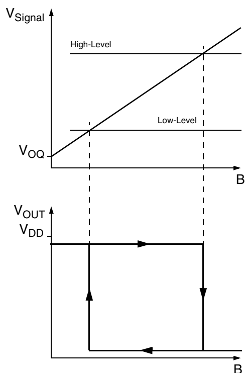
Fig. 2-4: HAL 1000 with unipolar behavior
