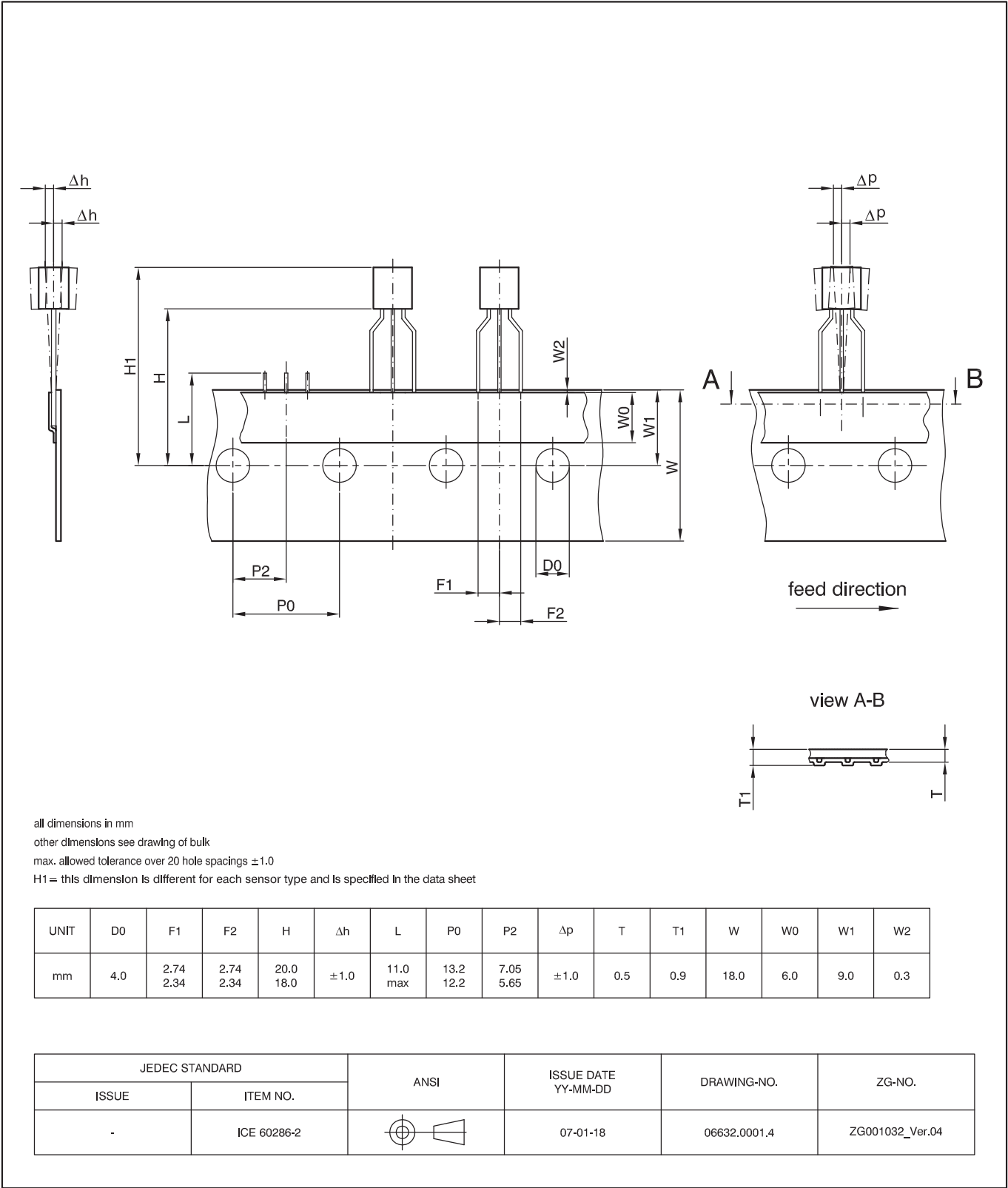
Fig. 3-4: TO92UT-1: Dimensions ammpack inline, spread Dimensions of Sensitive Area
