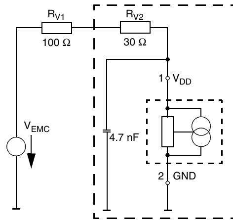
Fig. 5–3: Recommended EMC test circuit
