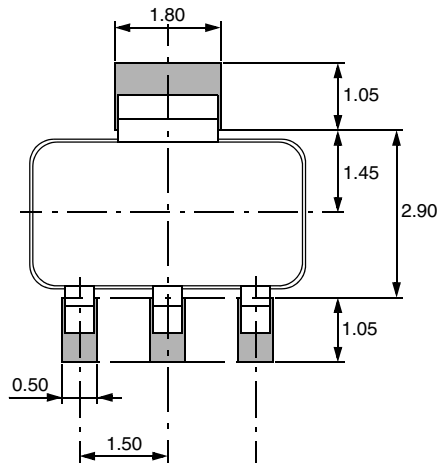
Fig. 3–4: Recommended footprint SOT89B-3, Dimensions in mm All dimensions are for reference only. The pad size may vary depending on the requirements of the soldering process.
