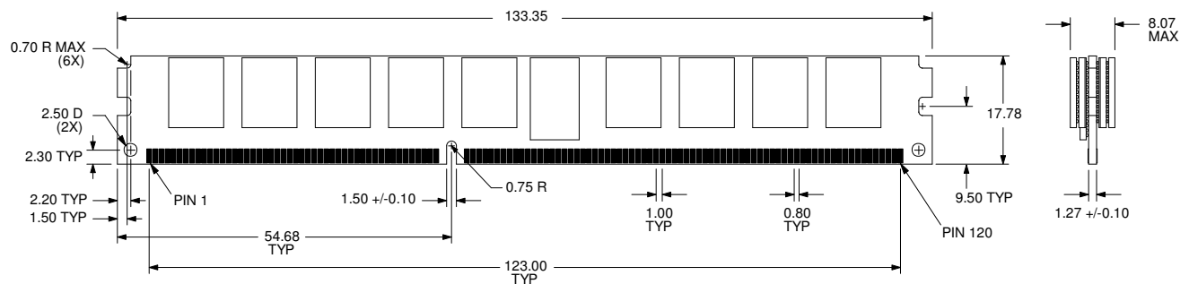
FRONT VIEW
