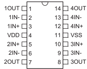
HT9294 14 DIP-A/SOP-A
