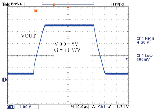
Fig 5. Large-Signal, Non-Inverting Pulse Response
