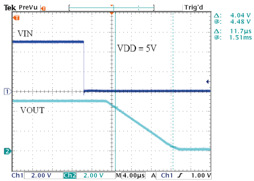
Fig 2. Slew Rate-Falling
