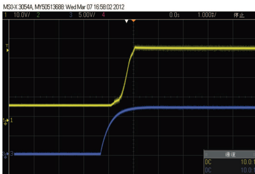
Start up Waveform (CH1=V OUT(AC) , CH2=V IN(AC) )
