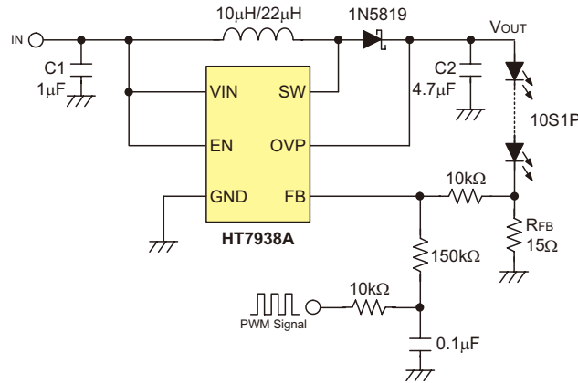
Fig.16 Application for Dimming Control Using a Filtered PWM Signal
