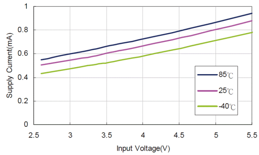
Fig.6 Supply Current VS Input Voltage
