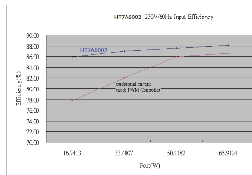
Figure 8. Efficiency Comparison between HT7A6002 & Traditional Current Mode PWM Controller (Measured at HT7A6002 Demo Board)
