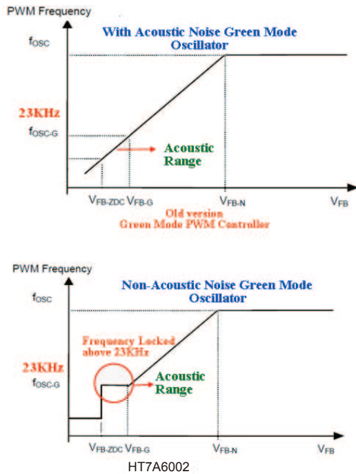
Figure 9. Oscillator Behavior Compared with HT7A6002 and other Green Mode PWM Controller
