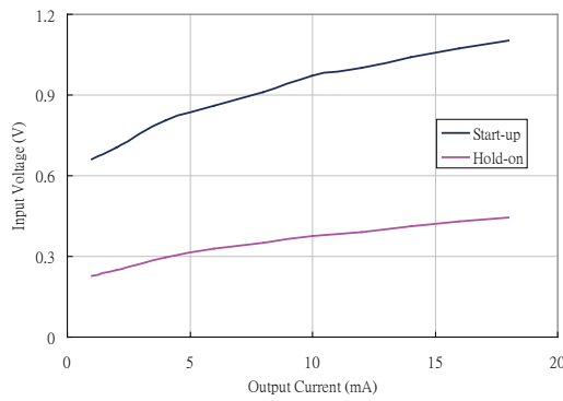
Fig 25. HT7730S Start-up & Hold-on Voltage
