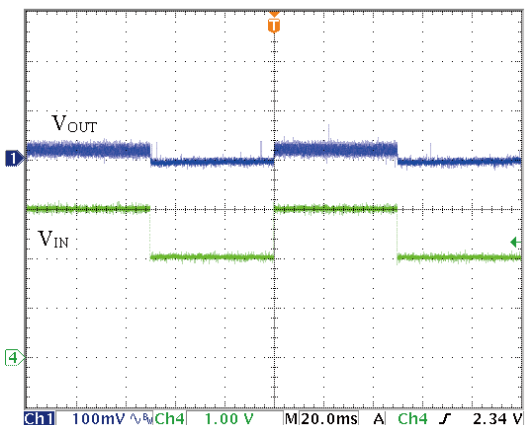
Fig 6. HT7750S Line Transient Response (L= 10 \mu H, C IN = C OUT = 10 \mu F, V IN = 3.0V)
