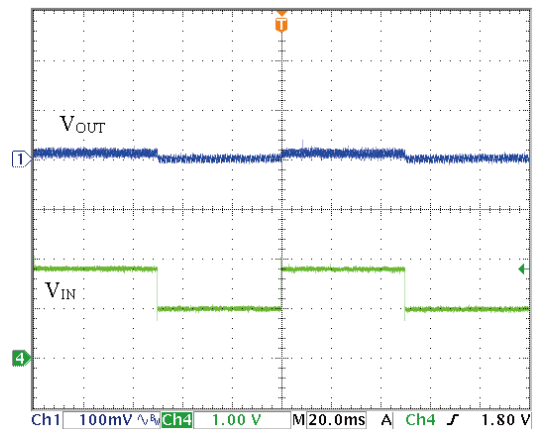
Fig 28. HT7730S Line Transient Response ( L=10\mu\text{H} , C_{\text{IN}}=C_{\text{OUT}}=10\mu\text{F} , V_{\text{IN}}=1.8\text{V} )
