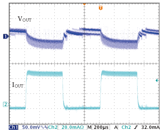
Fig 5. HT7750S Load Transient Response (L= 10 \mu H, C IN = C OUT = 10 \mu F, V IN = 3.0V)
