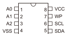
HT24LC256 8 DIP-A/SOP-A/TSSOP-A
