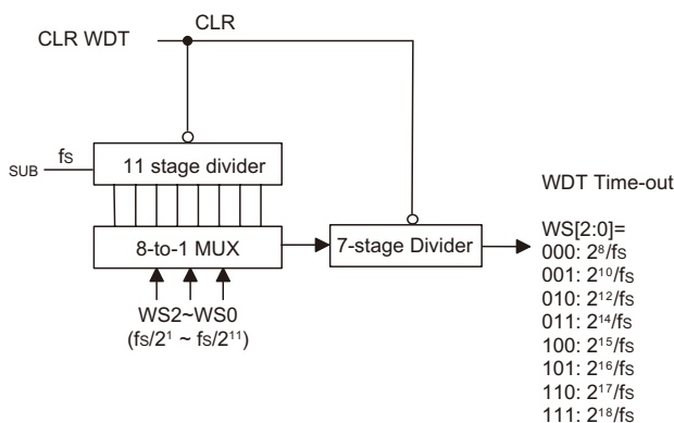
Watchdog Timer
