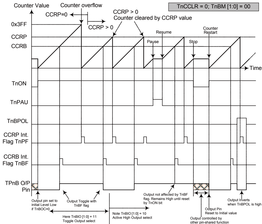
ETM CCRB Compare Match Output Mode – TnCCLR=0
