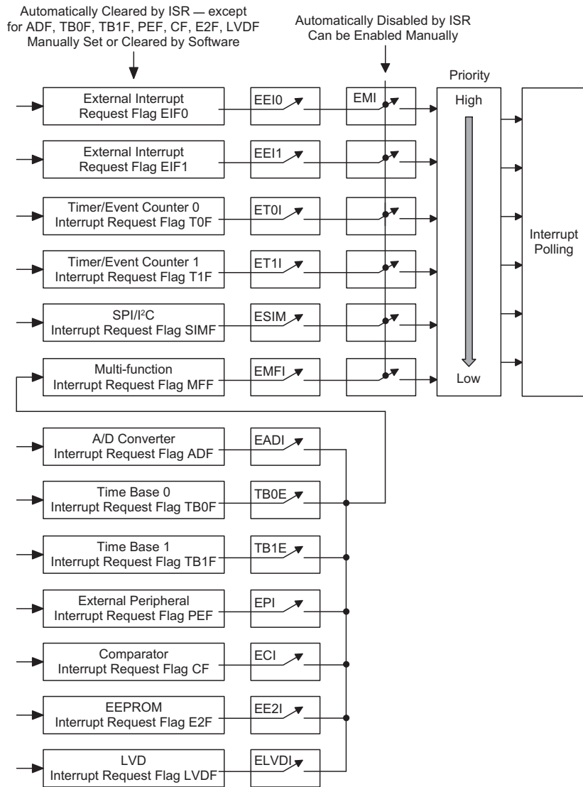
Interrupt Structure
