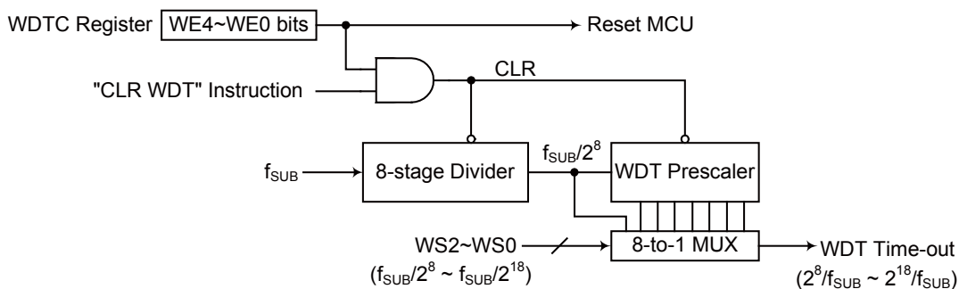
Watchdog timer
