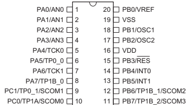
HT66F15 20 DIP-A/SOP-A/SSOP-A
