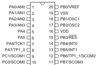
HT66F13 20 DIP-A/SOP-A/SSOP-A
