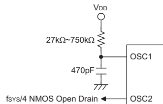
RC Oscillator
